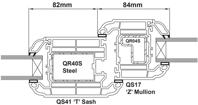
Optima Sculptured (84mm Mullion) Locking onto Mullion
