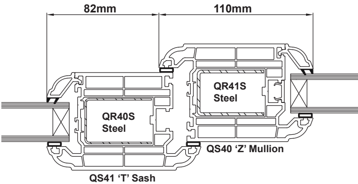
Optima Sculptured (110mm Mullion) Hinged off Mullion
