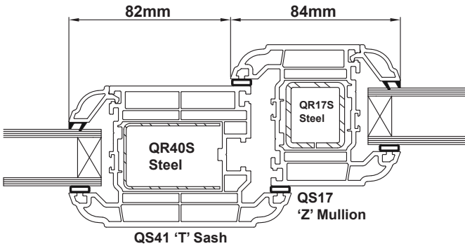
Optima Sculptured (84mm Mullion) Hinged off Mullion
