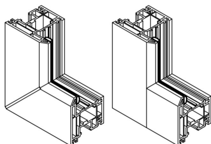
Traditional Welded Joint
